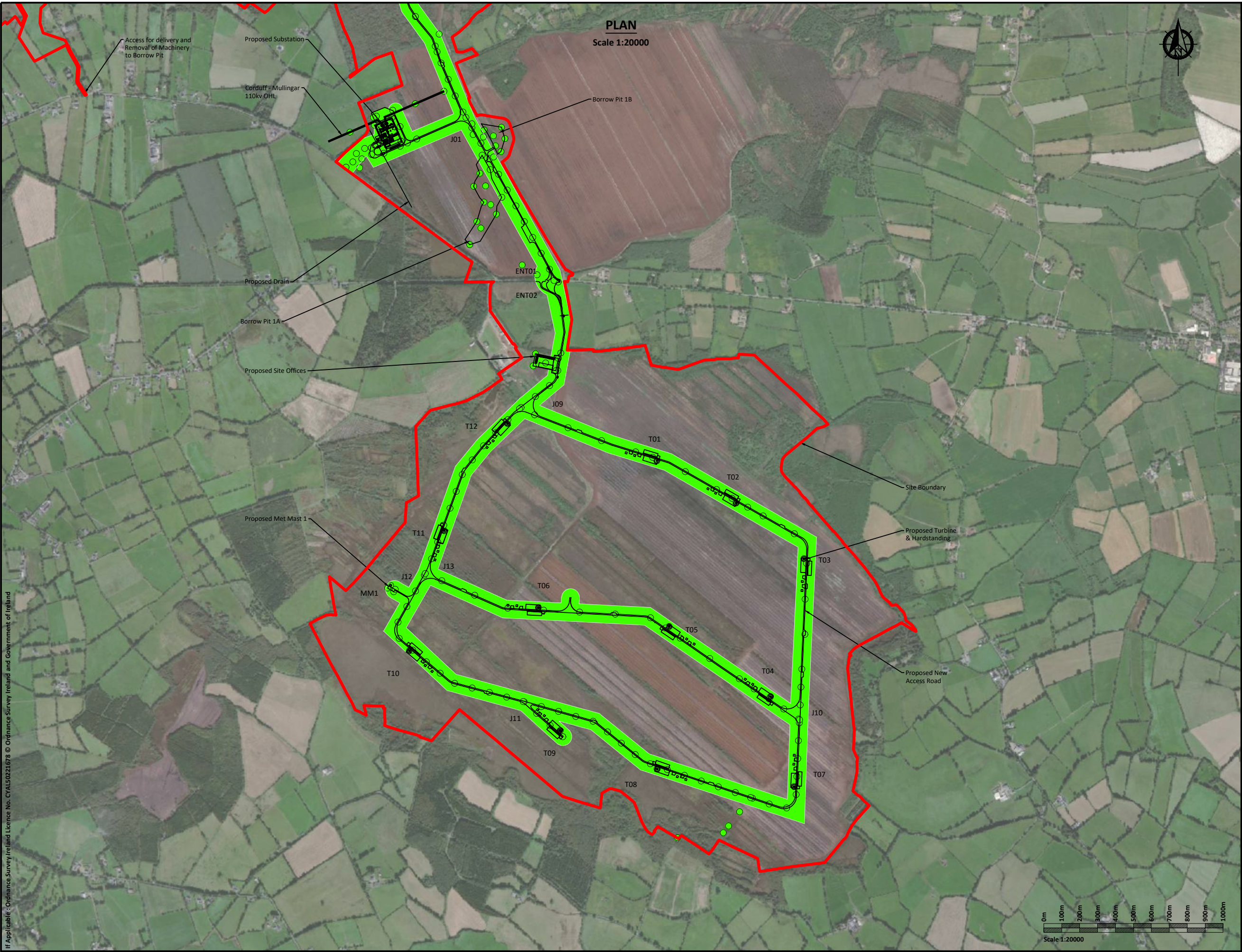
FIGURE 7.1 - FACTOR OF SAFETY PLAN SHEET 2 OF 2
