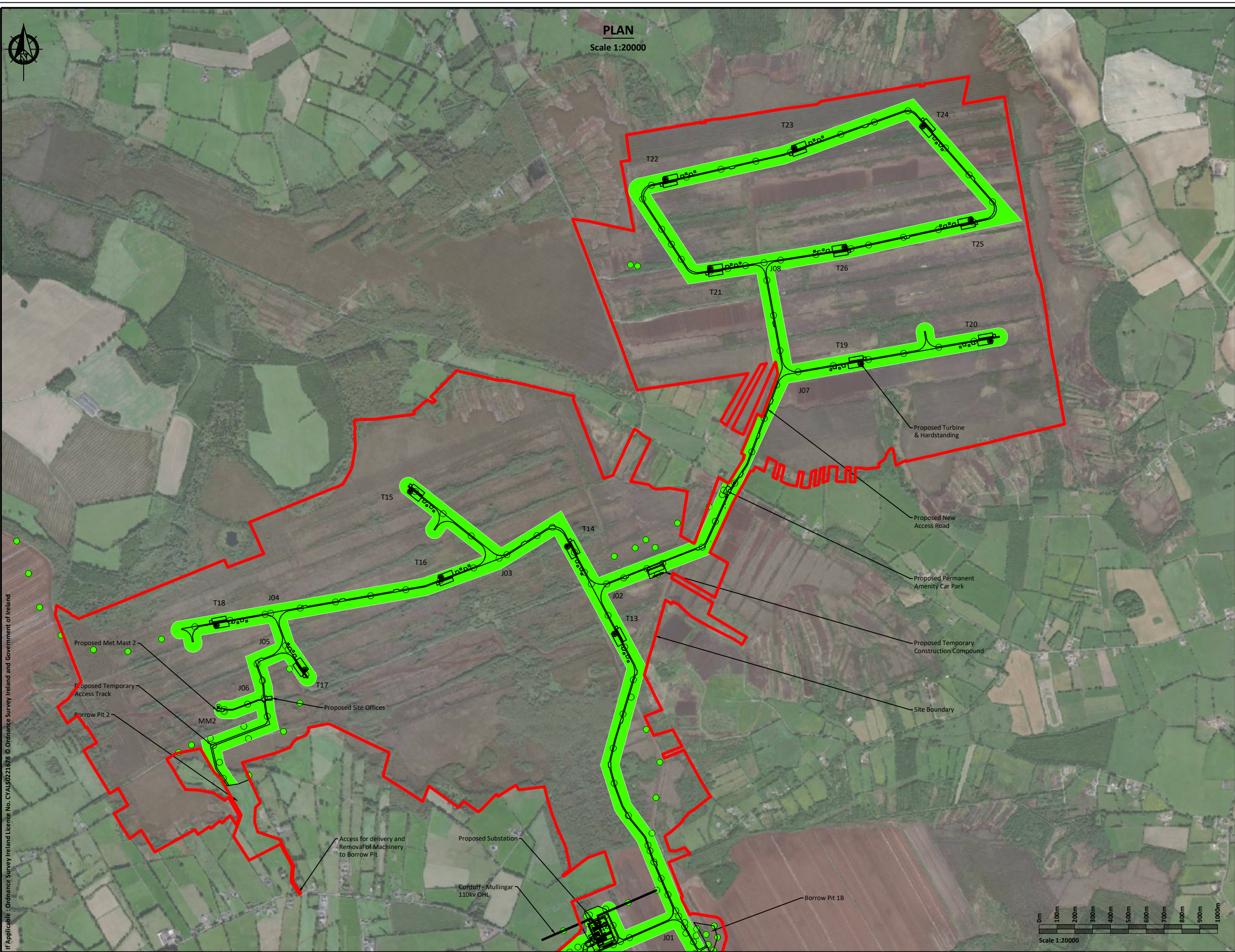
FIGURE 7.1 - FACTOR OF SAFETY PLAN SHEET 1 OF 2
